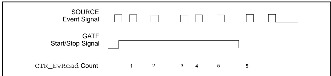
Figure 3-29. Timer Event Counting
