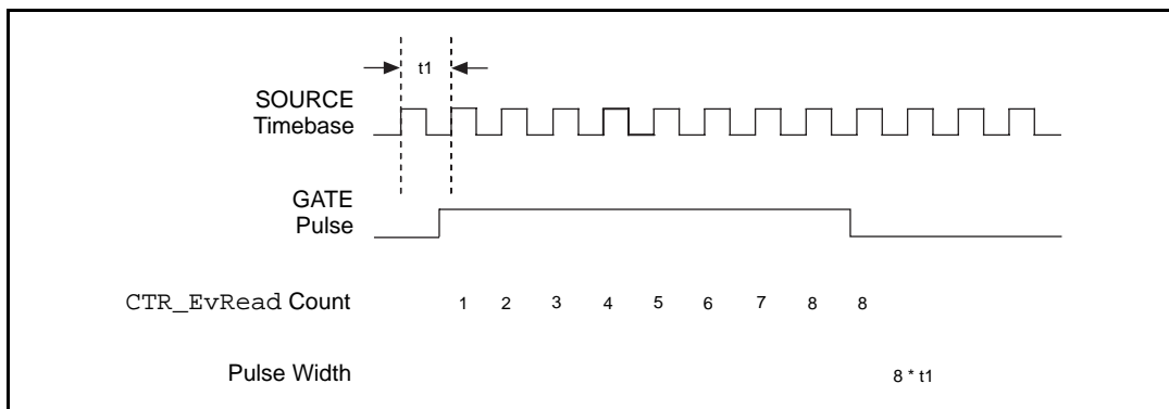
Figure 3-30. Pulse-Width Measurement
